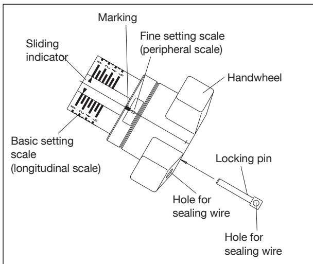
Handwheel
