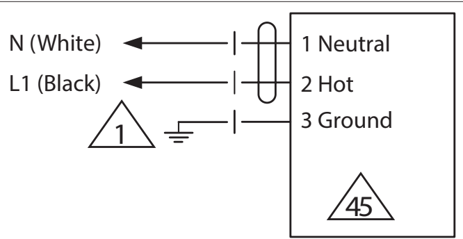
120 VAC
