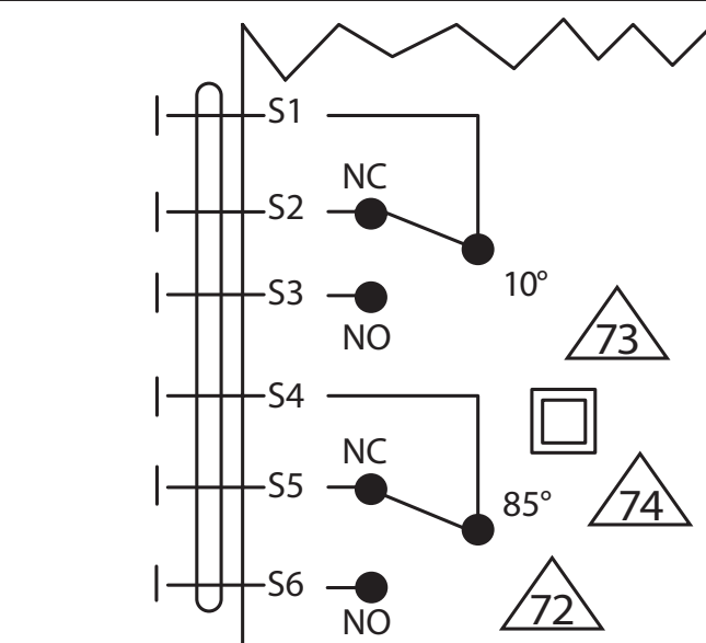
Auxiliary Switch
